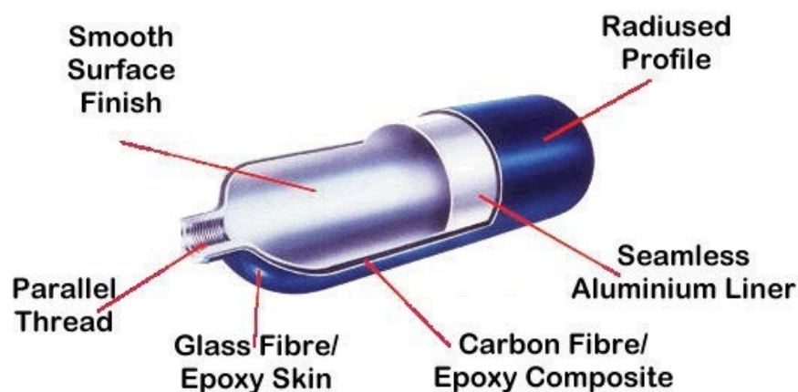
Figure 1: Typical Carbon Composite Cylinder
