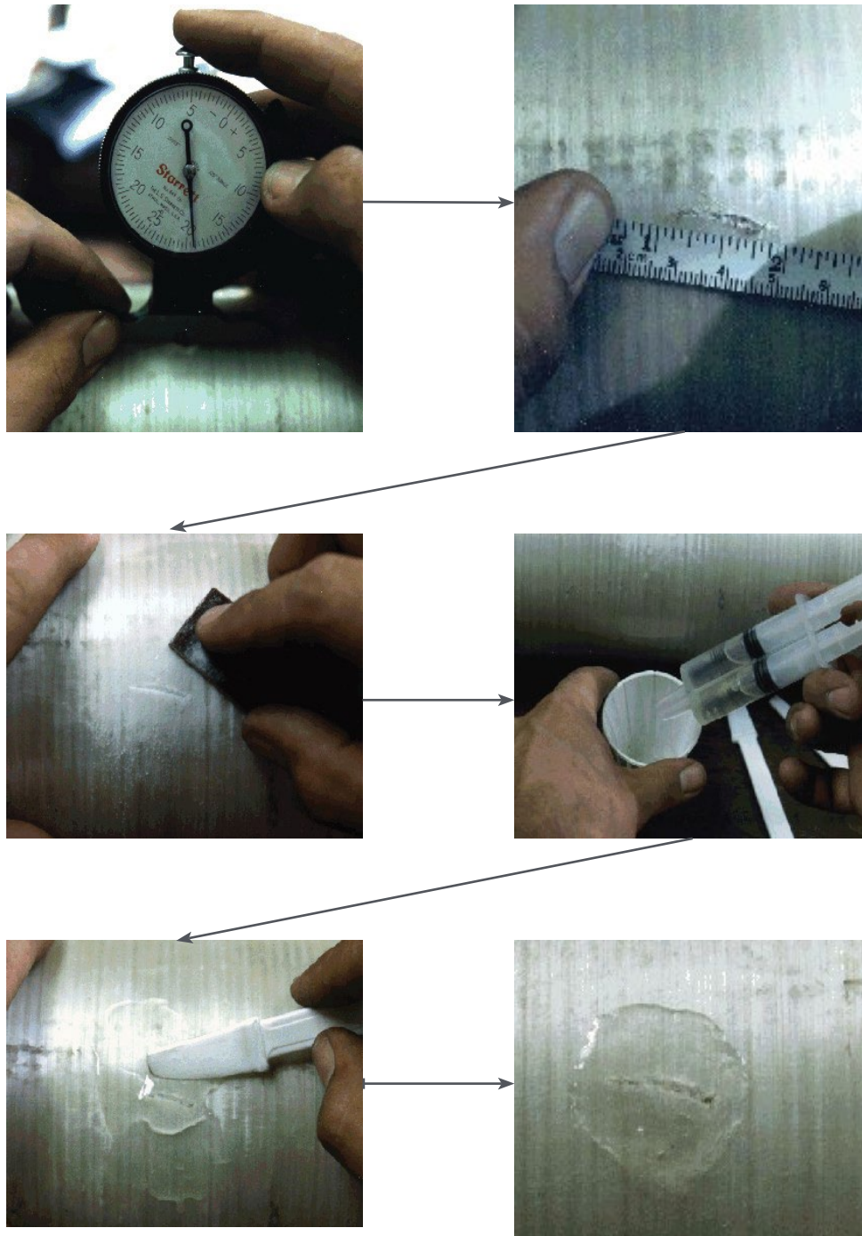
Figure 12: Typical Repair Sequence
