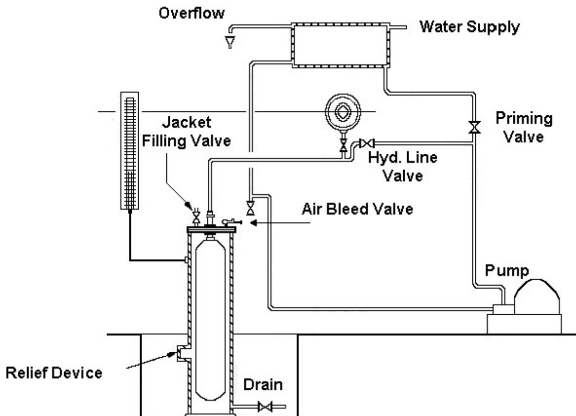
Figure 13: Water Jacket Volumetric Expansion Test (Fixed Burette)
